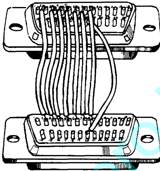
STANDARD CABLE
