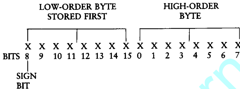
Figure 6-3. Integer Storage
